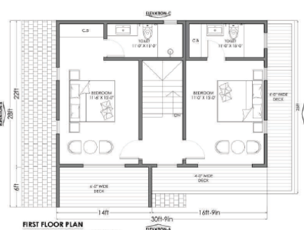
FIRST FLOOR PLAN COVERED AREA = 733 Sq.Ft DECK AREA = 187 Sq.Ft
